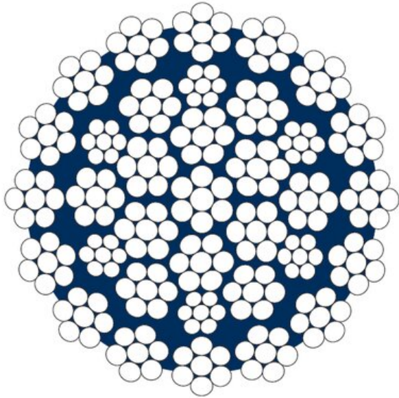
Tower crane
